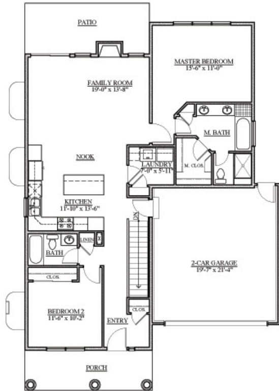
MAIN LEVEL FLOOR PLAN - 1358 Sq. Ft.
