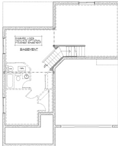
BASEMENT FLOOR PLAN 923 Sq Ft
