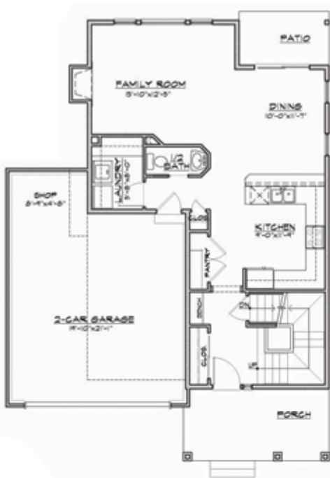
MAIN LEVEL FLOOR PLAN 849 Sq Ft
